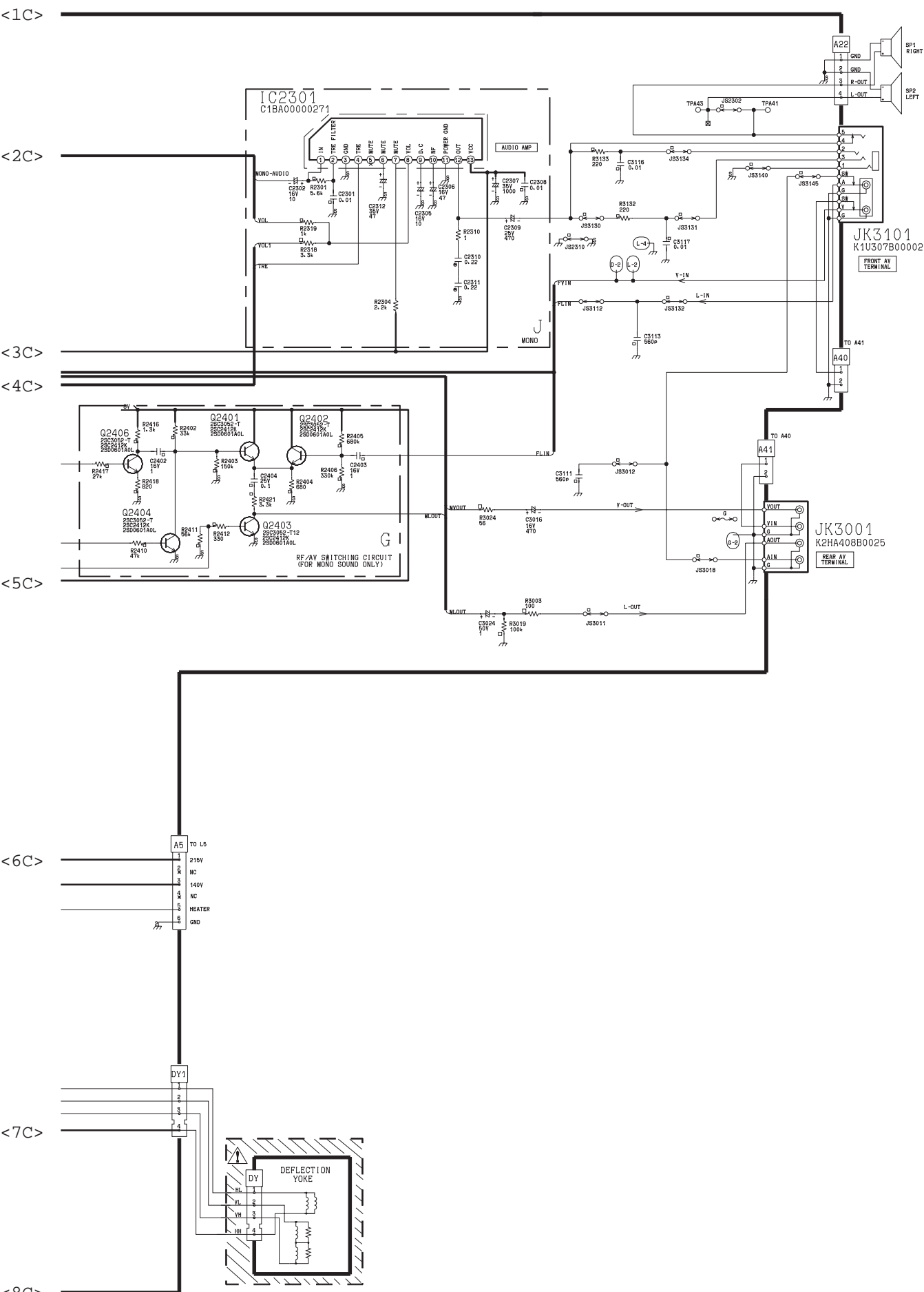
TC-21S85RQ A-Board (4 of 4) Schematic Diagram
