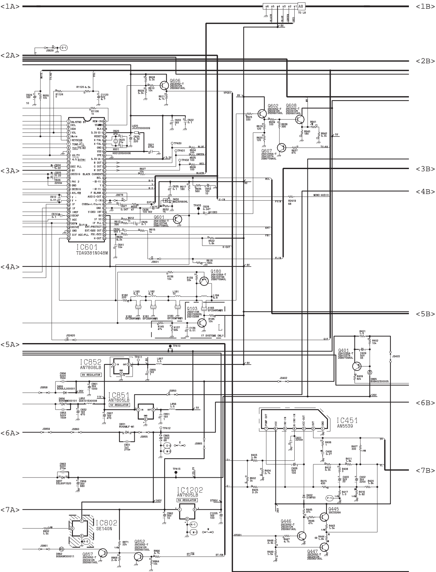
<8A> TC-21S85RQ A-Board (2 of 4) Schematic Diagram
