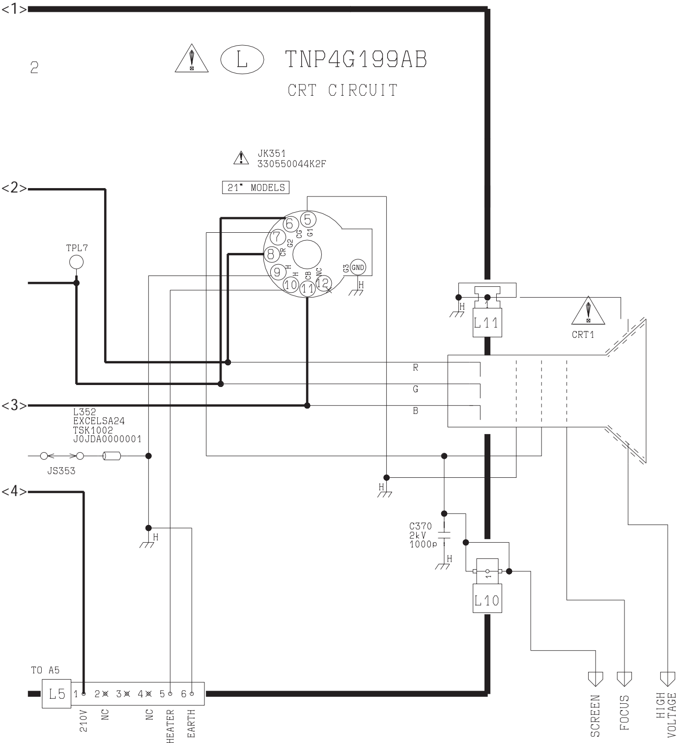
TC-21S85RQ L-Board (2 of 2) Schematic Diagram
