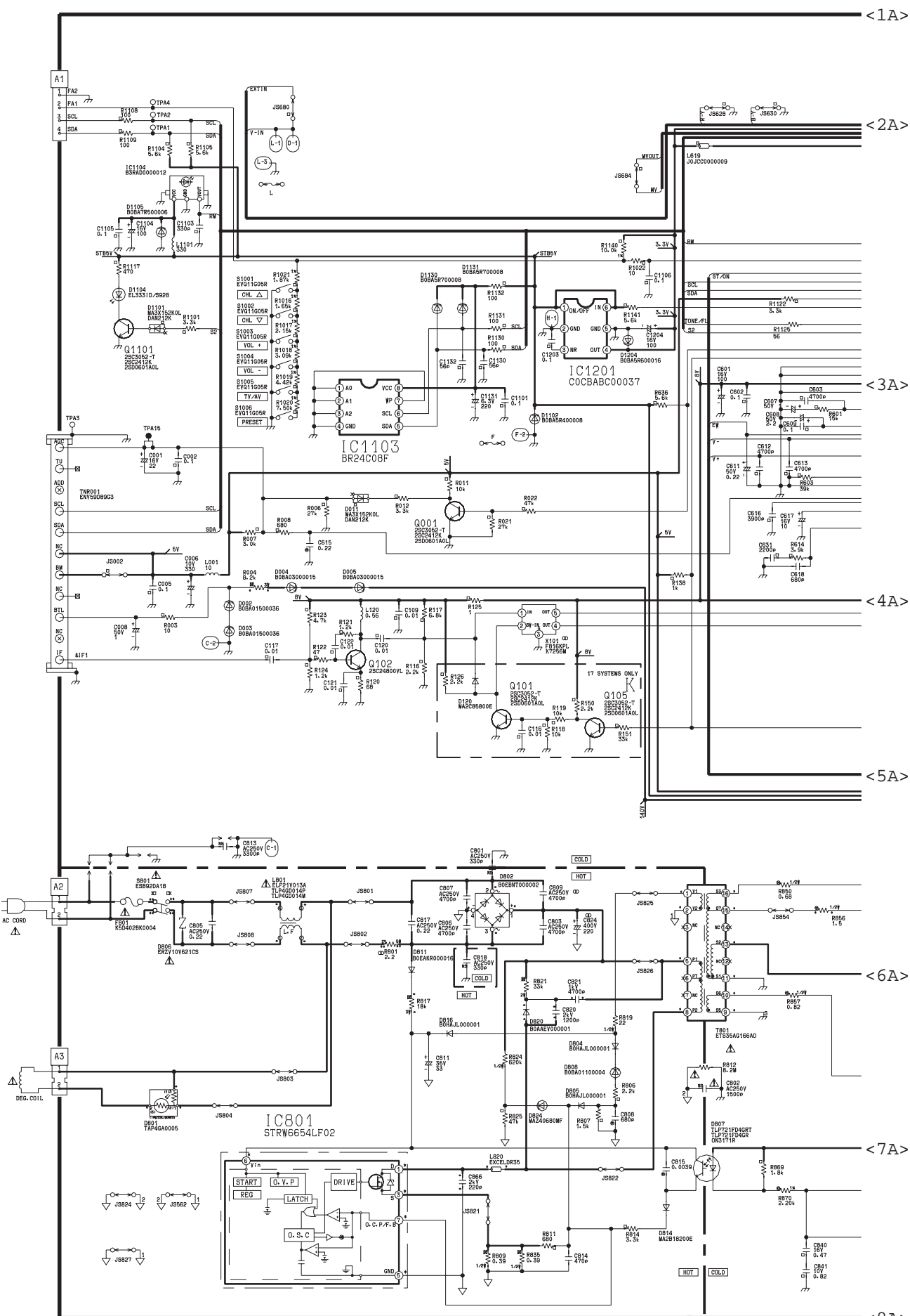
TC-21S85RQ A-Board (1 of 4) Schematic Diagram
